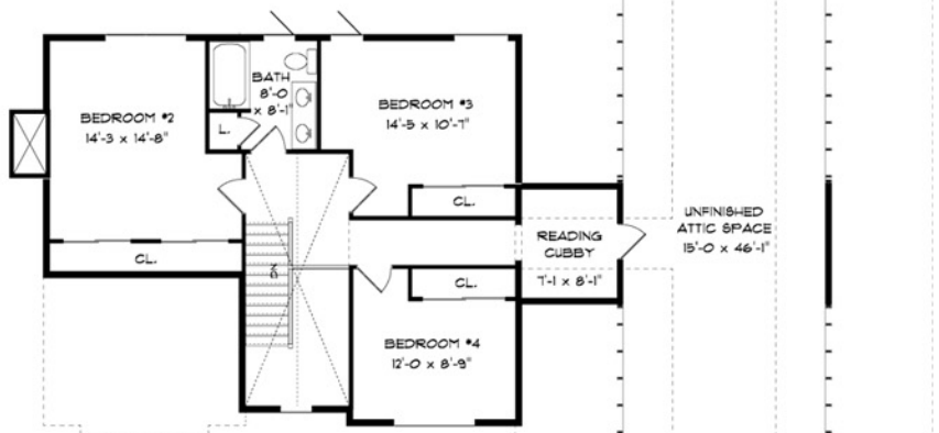
SECOND FLOOR 831 SQUARE FEET
